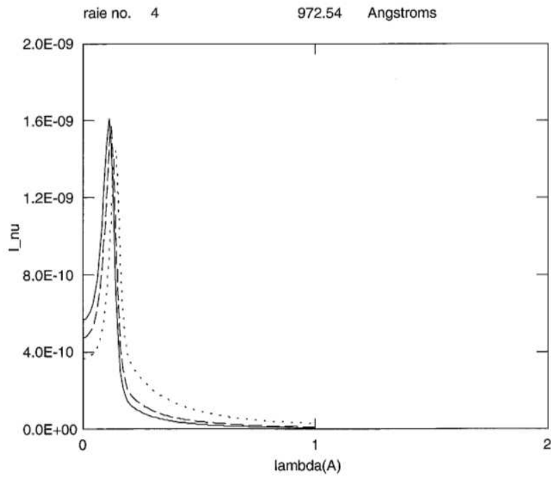
Figure 17: Half-profile of L\gamma line at 972Å
