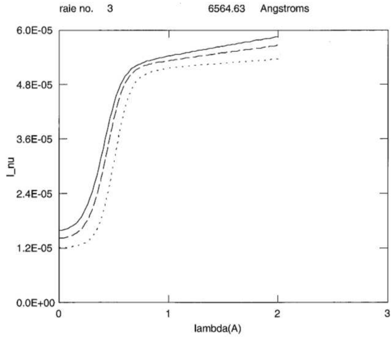
Figure 16: Half-profile of H\alpha line at 6564Å
