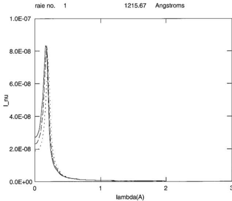
Figure 4: Half-profile of L\alpha line at 1215Å
