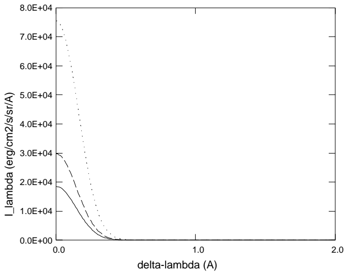
line 2 4 ( 4862 A ), E = 6.60E+03
