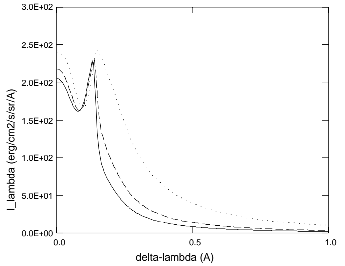
line 1 4 ( 972 A ), E = 1.68E+01
