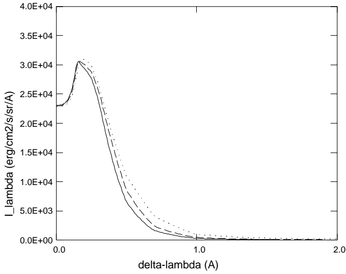
line 2 3 ( 6564 A ), E = 5.60E+04
