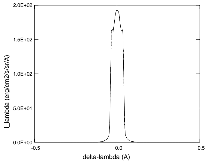
transition 11 ( 537 A ) , E = 1.48E+01 V(km/s) = 0
