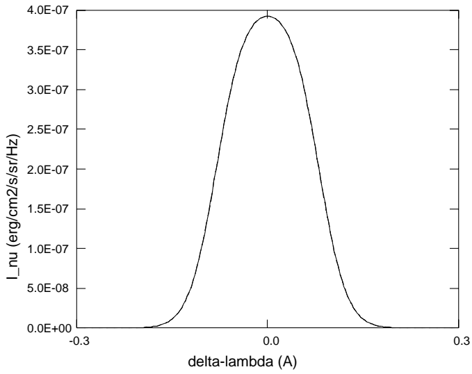
line 2 6 ( 3934 A ) , E = 1.77E+04 V(km/s) = 0
