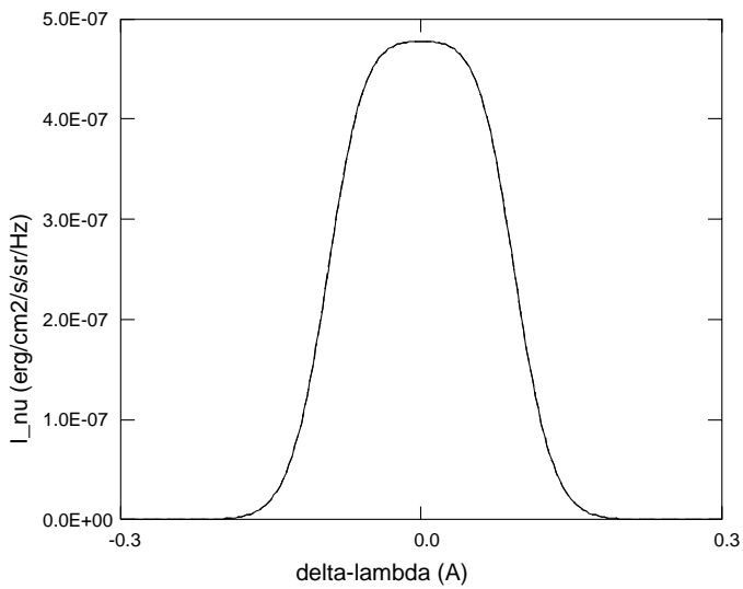
line 4 6 ( 8544 A ) , E = 1.10E+03 V(km/s) = 0
