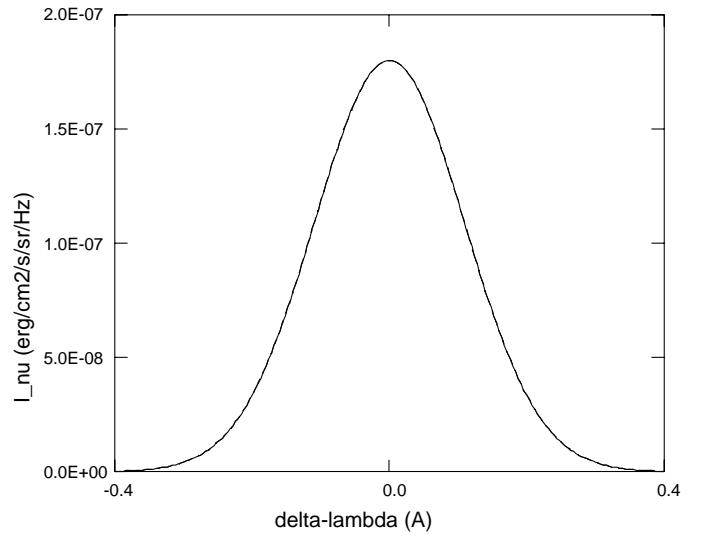
line 3 6 ( 8500 A ) , E = 3.67E+02 V(km/s) = 120
