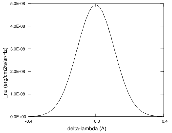
line 3 6 ( 8500 A ) , E = 1.26E+02 V(km/s) = 0
