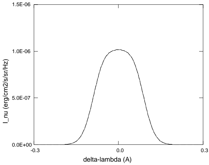
line 2 6 ( 3934 A ) , E = 3.74E+04 V(km/s) = 120
