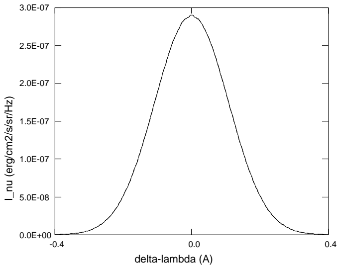
line 4 6 ( 8544 A ) , E = 3.21E+03 V(km/s) = 120
