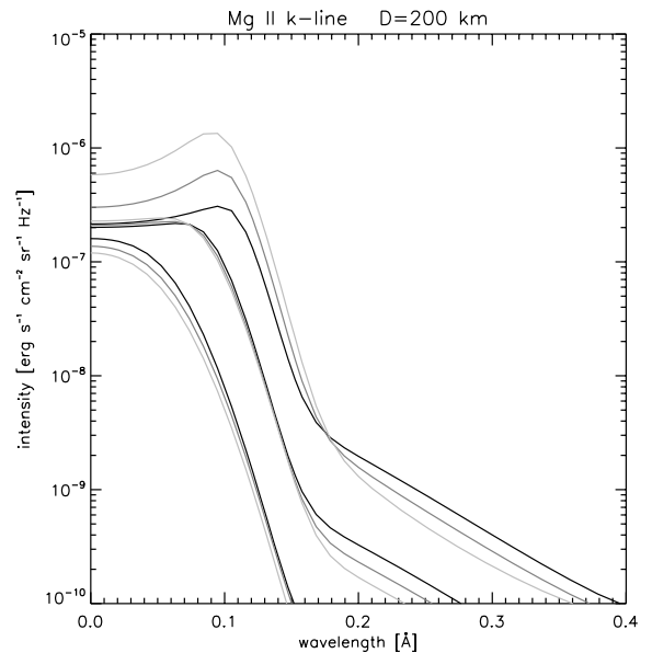
Fig. 2. Mg II k line profiles of the normally emergent radiation from slabs with D=200 km. The three sets of curves, increasing in their intensity, correspond to three gas pressures p=0.01, 0.1, and 0.5 dyne \text{cm}^{-2} . The gray scale corresponds to three temperatures: T=6000 K (black), 8000 K (dark gray), and 10000 K (light gray). Only one half of the symmetrical profiles is displayed.
