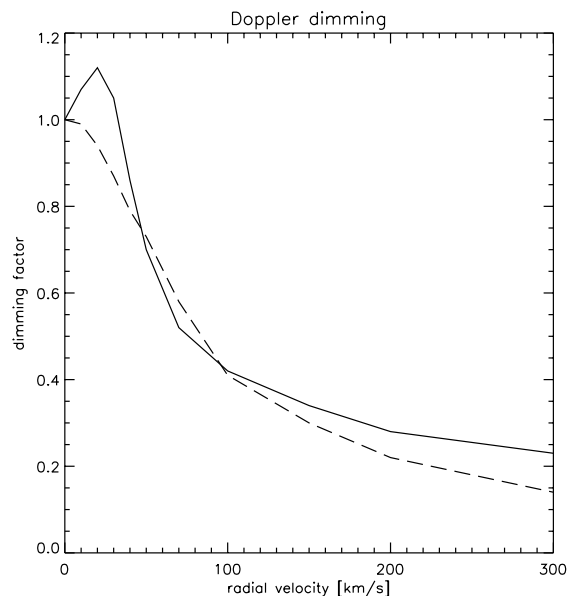
Fig. 9. Examples of the Doppler dimming effect on the Mg II k line. Shown is the dimming factor versus radial velocity, where the dimming factor is defined as the ratio of the line integrated intensity at a given velocity to the intensity at zero velocity. The plots correspond to models with D = 1000 km, T = 8000 K, p = 0.1 dyne cm -2 , and two different turbulent velocities of 5 km s -1 (full line) and 20 km s -1 (dashed line).
