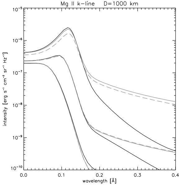
Fig. 6. Comparison between PRD and CRD profiles for D = 1000 km and T = 8000 K. Profiles with increasing intensity correspond to increasing gas pressures p = 0.001, 0.1 , and 0.5 \text{dyne cm}^{-2} . Black profiles correspond to PRD and gray ones to CRD having enhanced wings. For hydrogen, which determines the electron density, the PRD approach was used for Lyman \alpha and Lyman \beta lines. The gray dash then shows the effect of using CRD for both hydrogen and Mg II.
