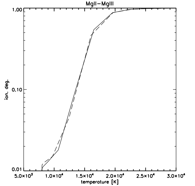
Fig. 7. Ionization degree Mg III/Mg II, as a function of the kinetic temperature for two PCTR models from Table 1. Full line for \gamma=10 and dashed line for \gamma=50 .
