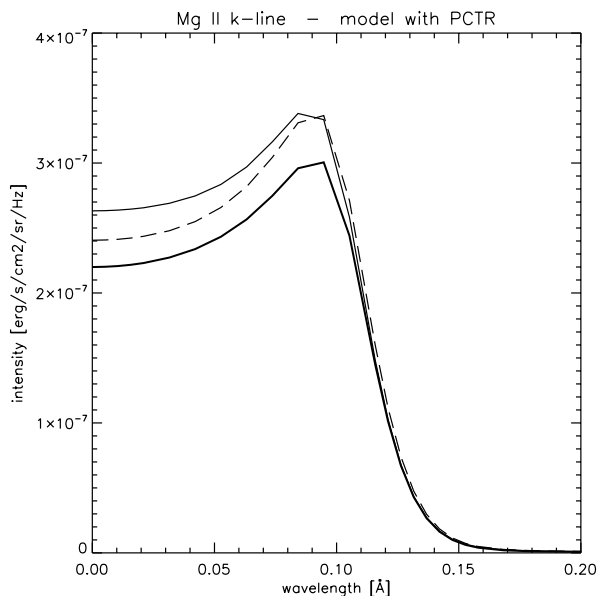
Fig. 8. Mg II k line profiles for two PCTR models from Table 1. The full thin line is for \gamma_{\text{tr}} = 10 and the dashed line for \gamma_{\text{tr}} = 50 . The thick line corresponds to an isothermal model with T = 8000 K.
