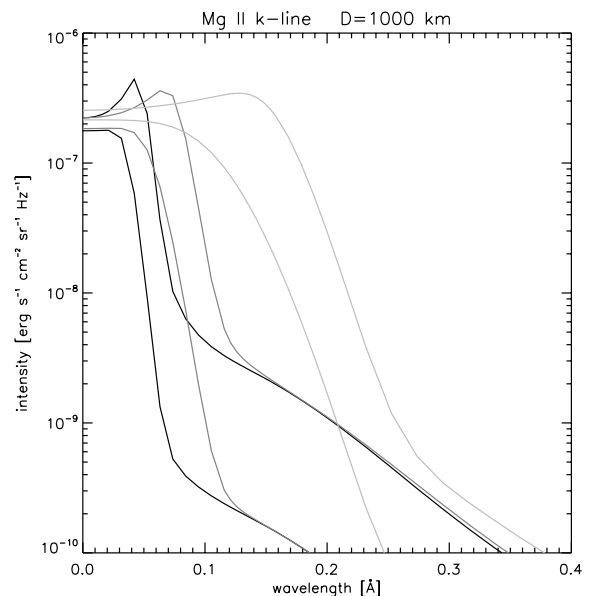
Fig. 5. Mg II k line profiles of the normally emergent radiation from the slab with D=1000 km and T=8000 K. The two sets of curves correspond to values of the gas pressure p=0.01 and 0.1 dyne cm -2 . For each pressure, three curves show an increasing line broadening for the three values of the microturbulent velocity: 0 km s -1 (black), 3 km s -1 (dark gray), and 8 km s -1 (light gray).
