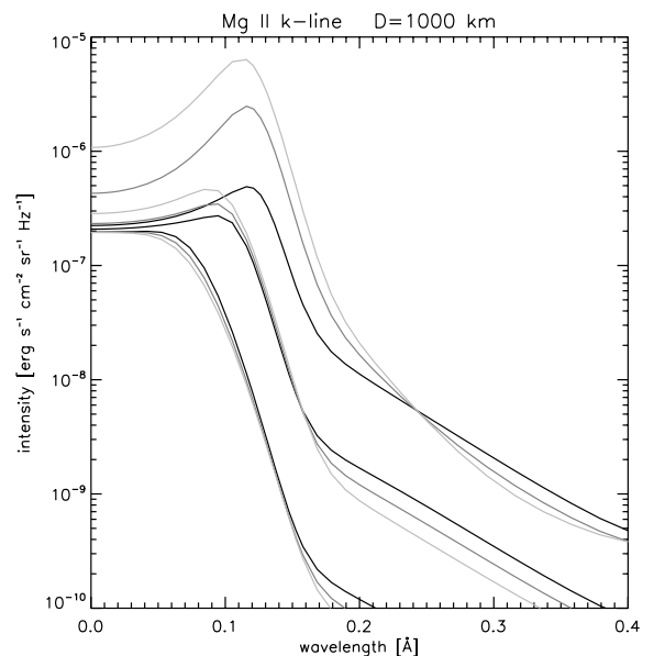
Fig. 3. Same as in Fig. 2, but for D = 1000 km.
