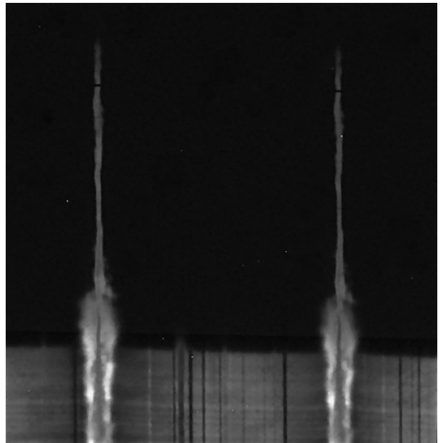
Fig. 1. Uncalibrated stigmatic spectra of the Mg II k (2795.53 Å) and h (2802.71 Å) lines detected by IRIS at 16:48:59 on July 18, 2013. The upper part of the Figure, where the profiles are narrow, corresponds to a prominence seen above the South Pole limb. The lower part of the Figure, where profiles are wide and reversed, corresponds to the chromosphere close to (and just above) the limb. The spectrum starts (left) at 2792.78 Å and ends (right) at 2805.34 Å. The spatial extension is 85 arcsec. Courtesy A. Title - LMSAL).
