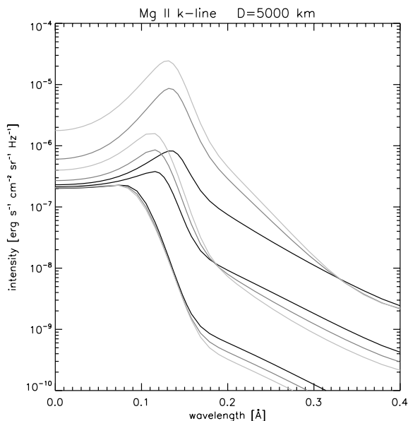
Fig. 4. Same as in Fig. 2, but for D = 5000 km. Note different intensity scale in this figure.
