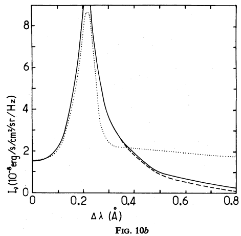
FIG. 10.—Comparison of CRD and PRD profiles (atmospheric model F). Full line , PRD with redistribution functions corresponding to the OSC approximation; dotted line , complete redistribution; dashed line , R_{ILA} redistribution function (scattering coherent in the rest frame of the atom). (a) L\alpha . (b) L\beta .
