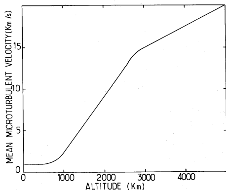
FIG. 2.—Mean microturbulent velocity versus altitude (model used in computations).
