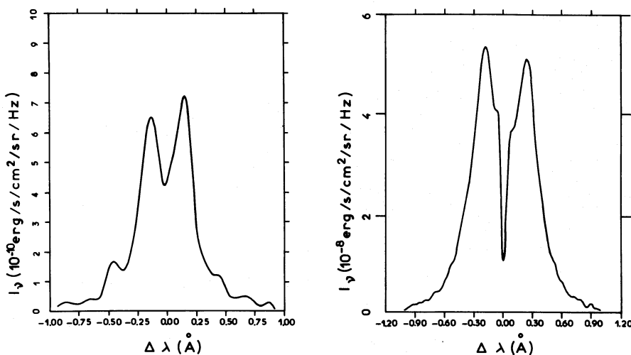
FIG. 1.—Observed profiles at the center of the solar disk. (a) L\beta . (b) L\alpha .
