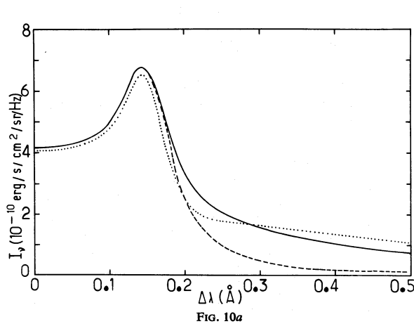
FIG. 10.—Comparison of CRD and PRD profiles (atmospheric model F). Full line , PRD with redistribution functions corresponding to the OSC approximation; dotted line , complete redistribution; dashed line , R_{ILA} redistribution function (scattering coherent in the rest frame of the atom). (a) L\alpha . (b) L\beta .
